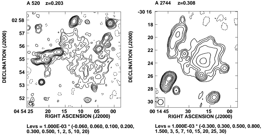
Figure 2: Left panel: The radio halo in A 520, imaged with a circular synthesized restoring beam with FWHM = 15'' . Right panel: Image of the radio halo in A 2744. The elongated emission in the NE peripheral region is a relic. The synthesized restoring beam is a circular Gaussian with a FWHM of 50'' .
